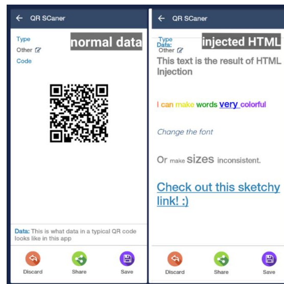
Figure 3 HTML injection
